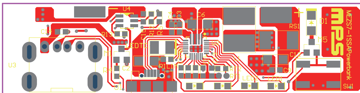
Figure 6: Top Layer
