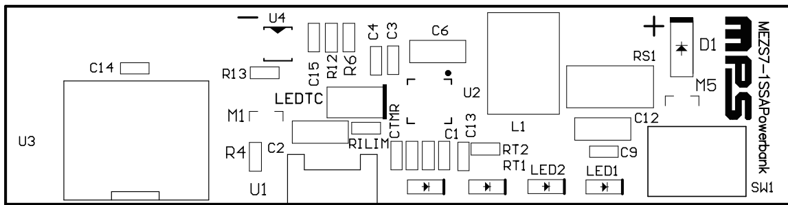
Figure 5: Top Silk
