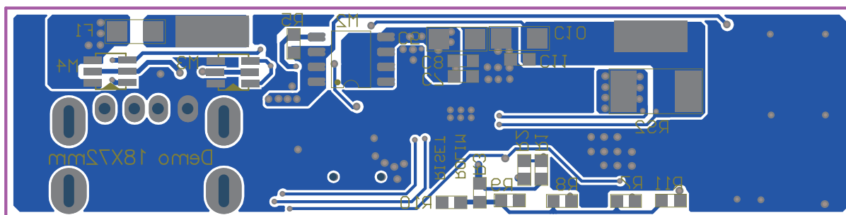
Figure 7: Bottom Layer
