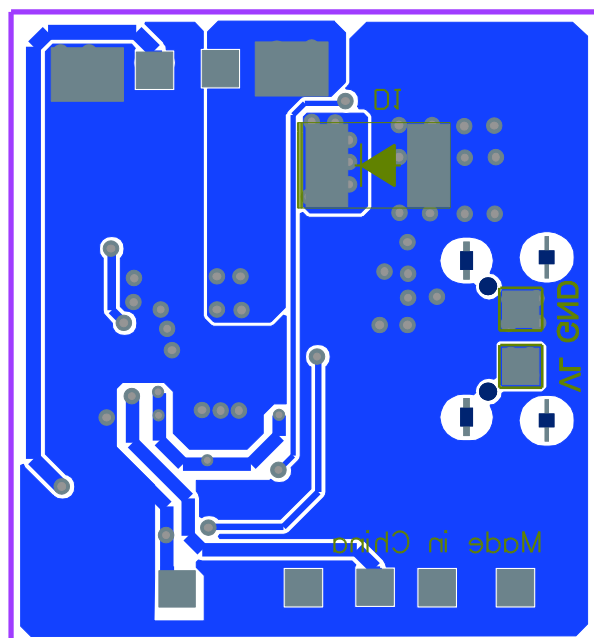
Figure 5: Bottom Layer
