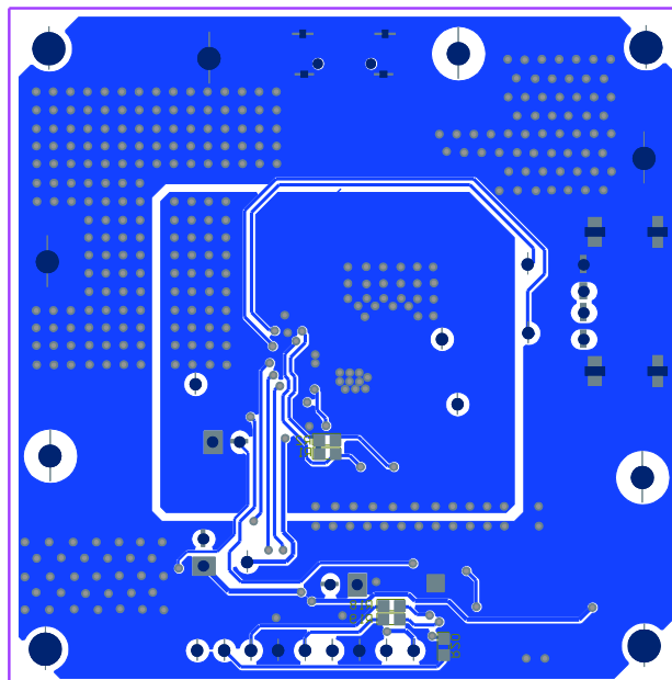
Figure 4: Bottom Layer
