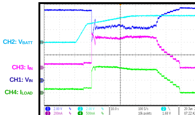
MPPT Behavior during Charging Cycle
