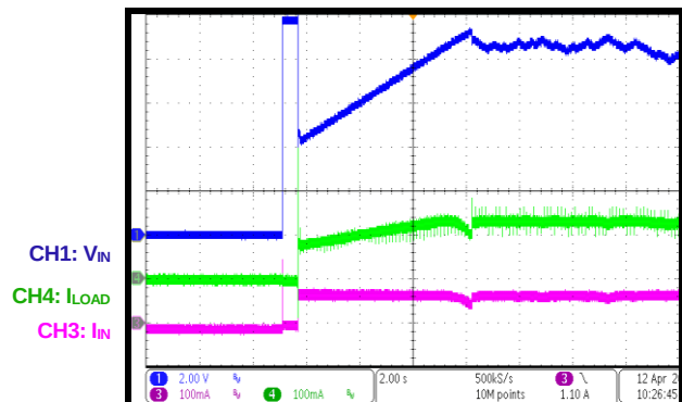
MPPT Process for PV Panel from Start-Up to Steady State
