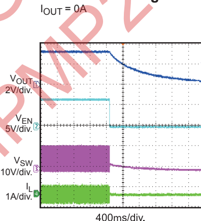
Shutdown through Enable I_{OUT} = 0A
