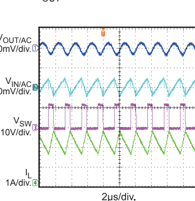
Input/Output Ripple I_{OUT} = 2A
