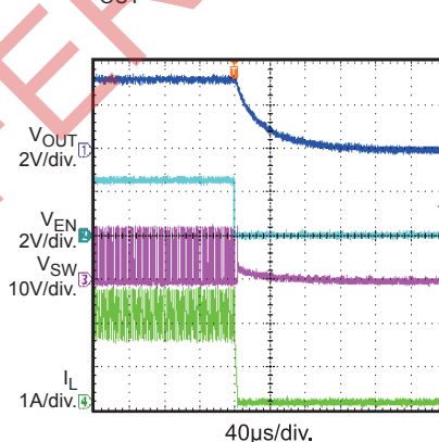
Shutdown through Enable I_{OUT} = 2A
