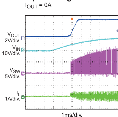
Startup through Input Voltage I_{OUT} = 0A
