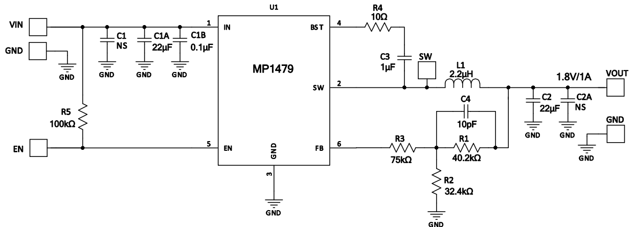
Figure 9: 12V IN , 1.8V/1A Output
