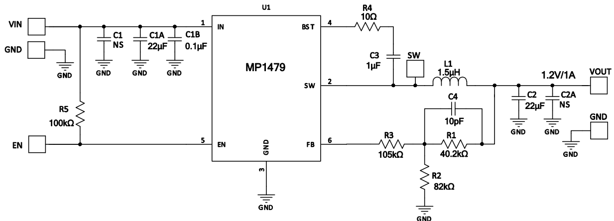
Figure 11: 12V IN , 1.2V/1A Output
