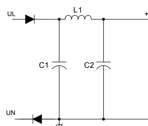
Figure 10: Half-Wave Rectifier
