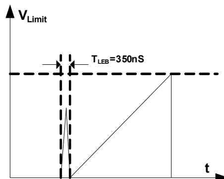
Figure 6: Leading-Edge Blanking
