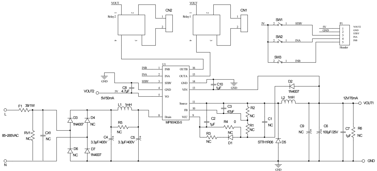
Figure 7: Typical Application with 12V/70mA, and 5V/50mA Output
