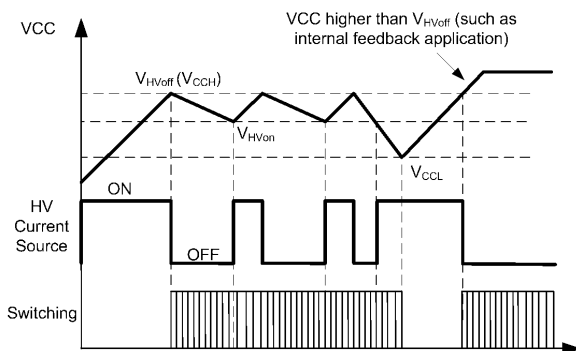
Figure 2: HV Current Source and VCC Operation
