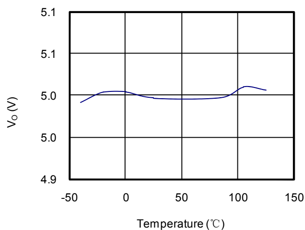
V_O (MP161x-5) vs. Temperature
