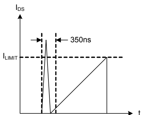
Figure 5: Leading-Edge Blanking
