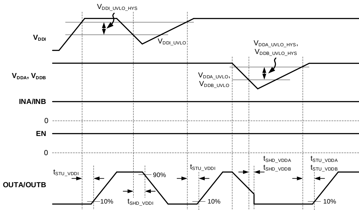
Figure 4: V DDI and V VDDA, VDDB Under-Voltage Lockout (UVLO)
