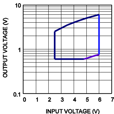
Operating Range
