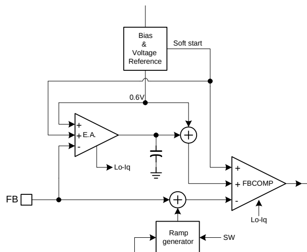
Figure 2: Operation Blocks at Sleep Mode
