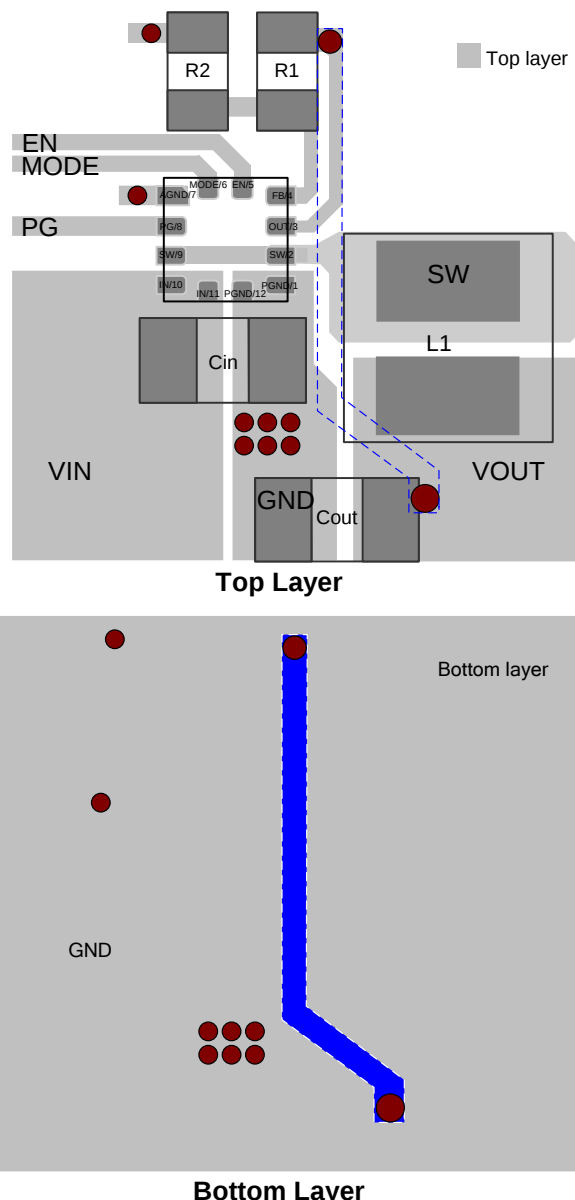
Bottom Layer Figure 7: Recommended Layout
