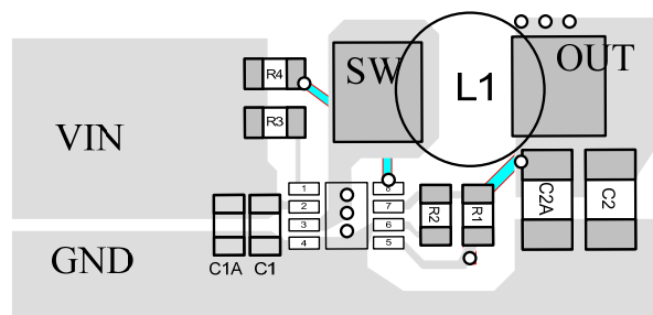
Figure 3: Layout Recommendation
