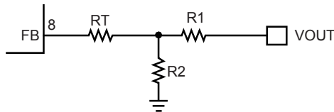
Figure 4— T-type Network
