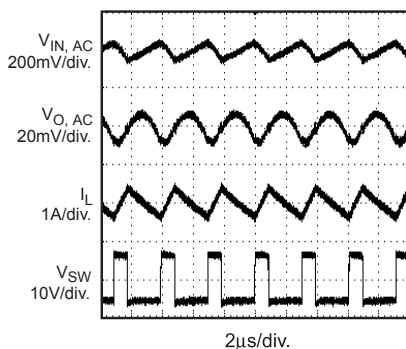
Full Load Operation
