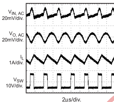
No Load Operation
