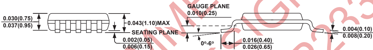
FRONT VIEW
