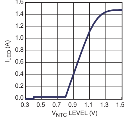
NTC Curve
