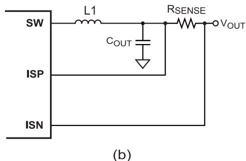
Figure 2—Current Sensing Methods
