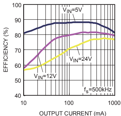
Efficiency @ V_{OUT}=2.5V
