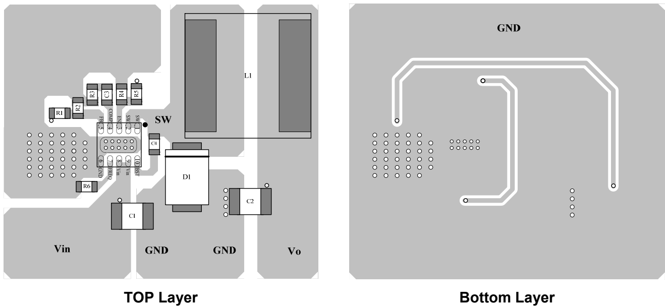
MP2562DQ Layout Guide Figure 6—MP2562 Typical Application Circuit and PCB Layout Guide
