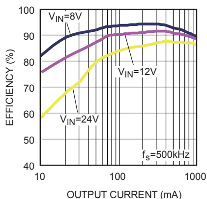
Efficiency @ V_{OUT}=5V
