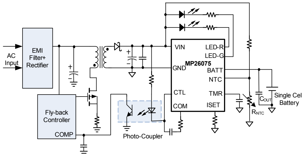
Figure 2— System Configuration
