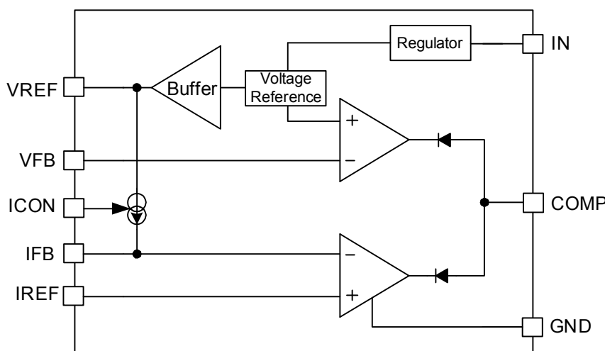
Figure 1—Block Diagram
