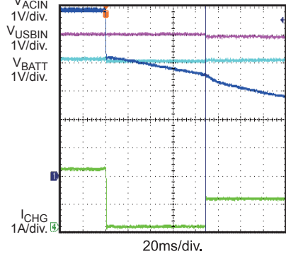
Short-Circuit Protection
