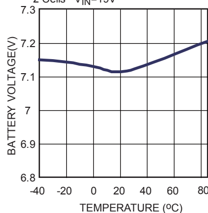
BATT Charge Full Voltage vs. Temperature
