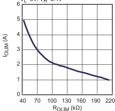
Programmable Output Current Limit, Discharge Mode
