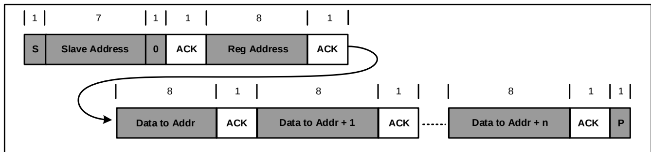
Figure 14: Multi-Write
