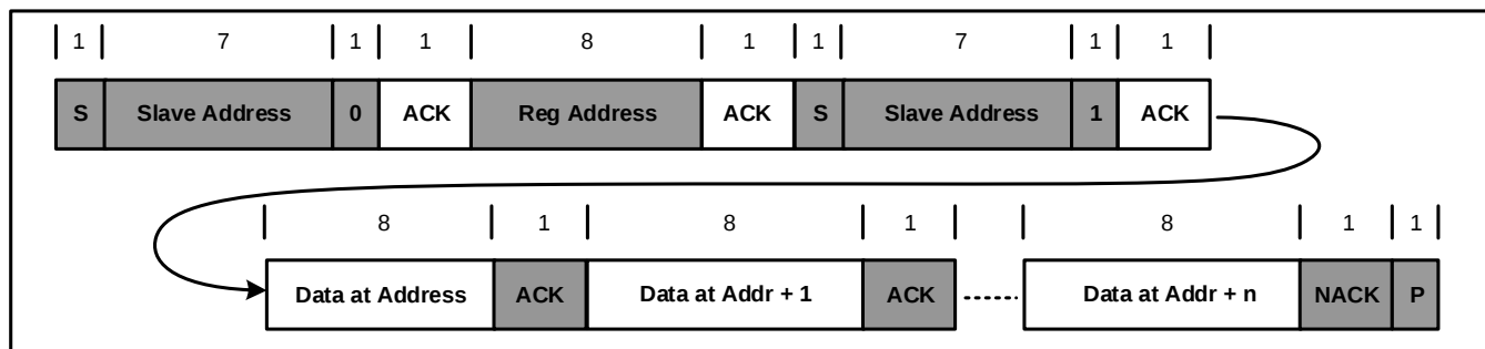
Figure 15: Multi-Read
