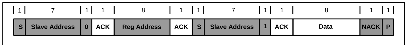
Figure 13: Single Read
