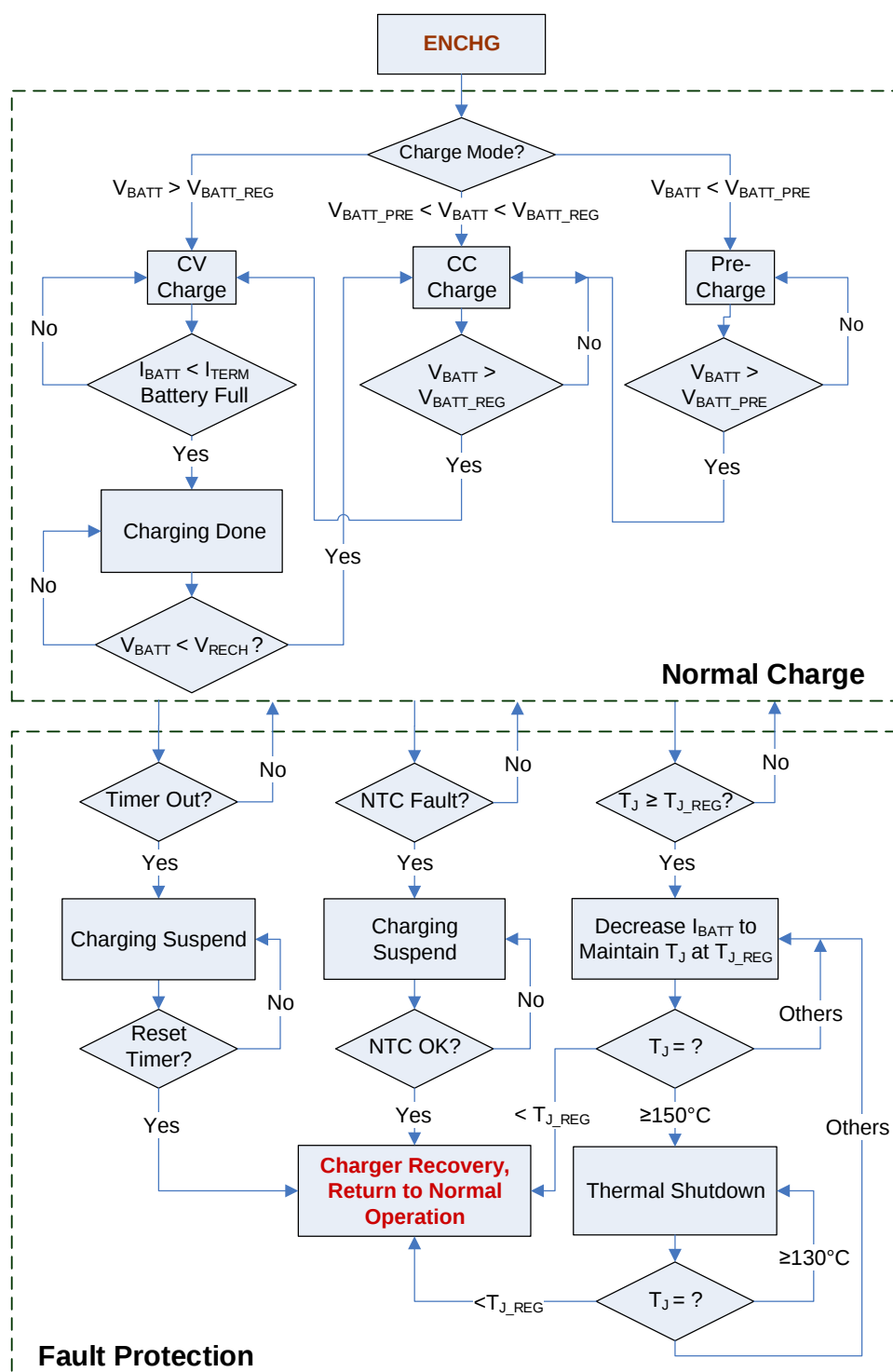
Figure 19: Charging Process
