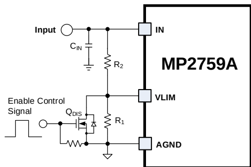
Figure 4: Enable Control
