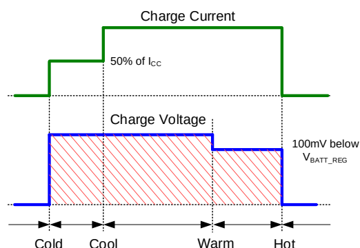
Figure 3: JEITA Protection
