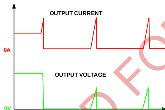
Figure 9—Over-current Behavior in HICCUP Mode. F_{sw} = 600\text{kHz}
