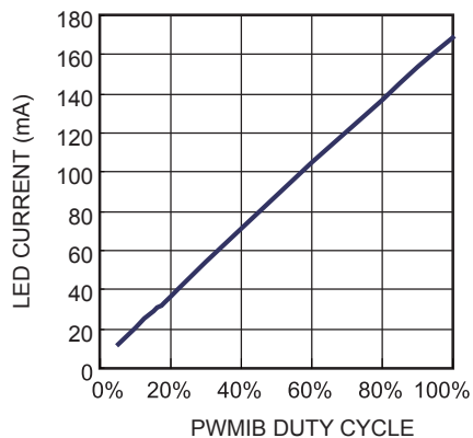
PWMIB Dimming Duty vs. WLED Current
