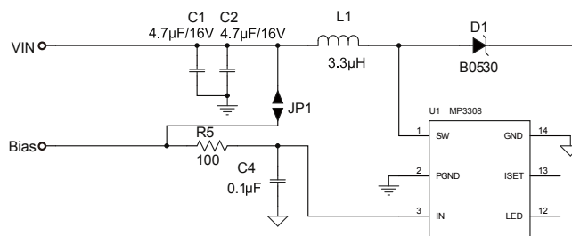
Figure 3—Input Bias Filtering
