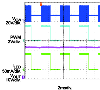
PWM Dimming f_{PWM}=200Hz , DPWM=50%
