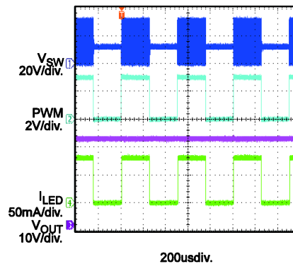
PWM Dimming f_{PWM}=2kHz , DPWM=50%
