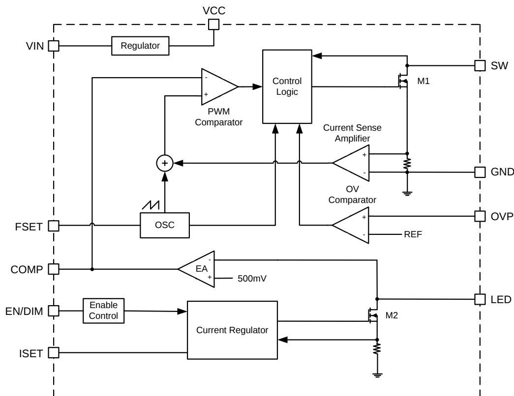
Figure 1—MP3310 Function Block Diagram
