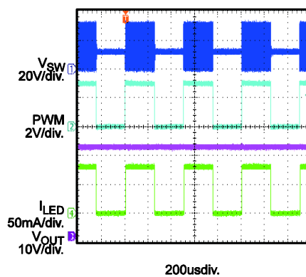
PWM Dimming
