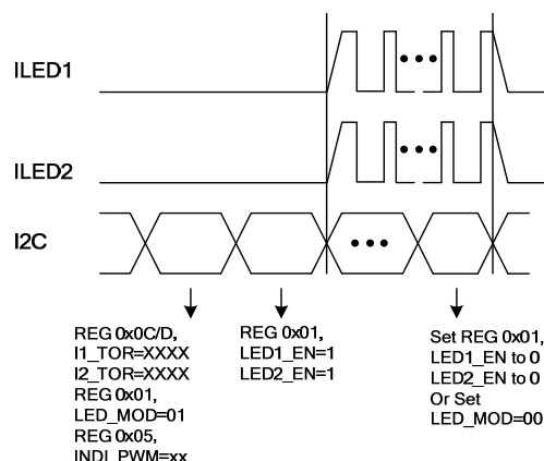
Figure 3: Indicator Mode
