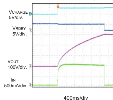
Charging Waveform
