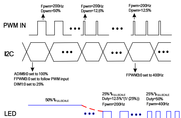
Figure 7: Mix Dimming from PWM Input
