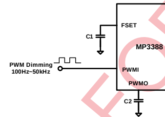
Figure 3—PWM Dimming with Internal Triangle Waveform Generator
