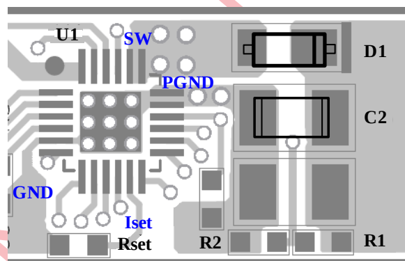
Figure 7—Layout Consideration
