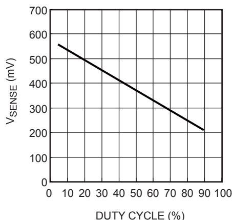
Figure 3— V_{SENSE} vs Duty Cycle
