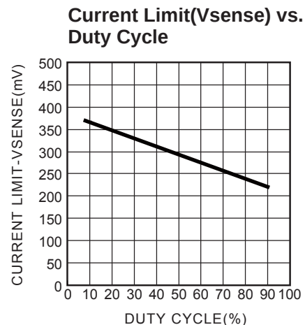
Figure 3— V_{SENSE} vs Duty Cycle
