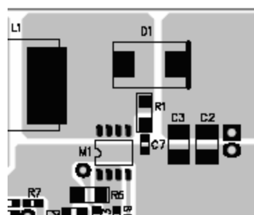
Figure 4—Layout Consideration
