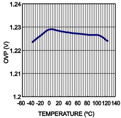
OVP Voltage vs. Temperature
