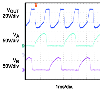
2.5V Input Operation: 80°C
