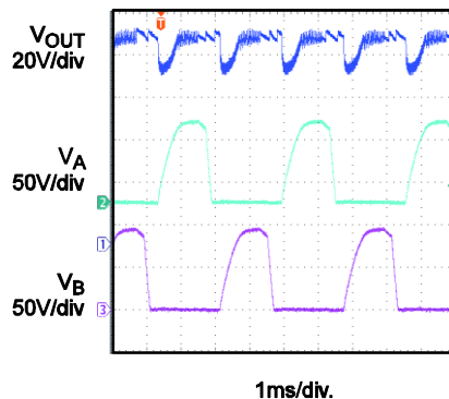
4.5V Input Operation: 80°C
