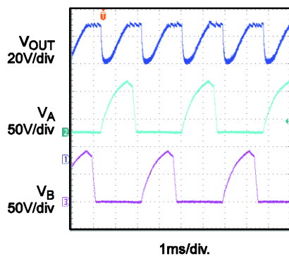
3.5V Input Operation: 80°C
