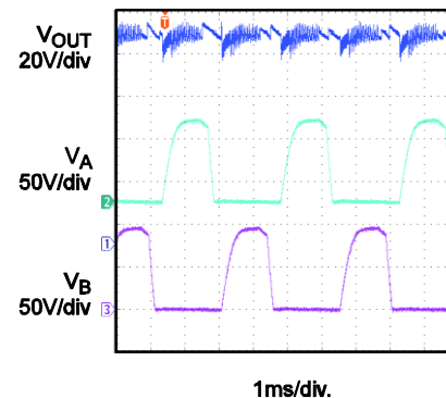
5.5V Input Operation: 80°C
