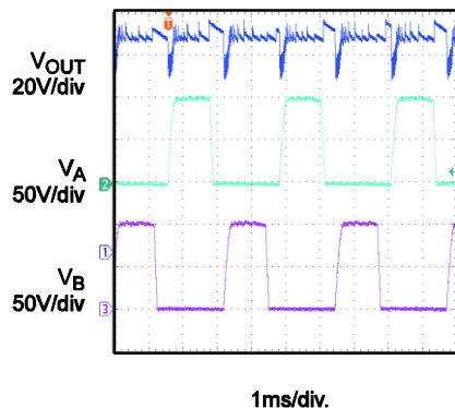
4.5V Input Operation: -40°C
