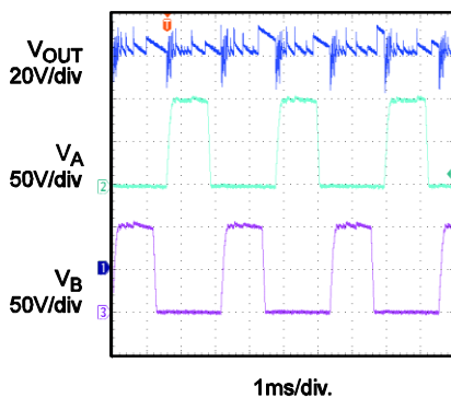
5.5V Input Operation: -40°C
