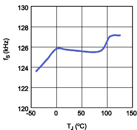
Switch Frequency vs. T_J
