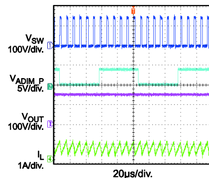
Pulse-input Analog Dimming
