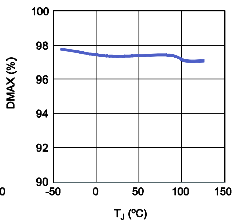
Maximum Duty vs. T_J
