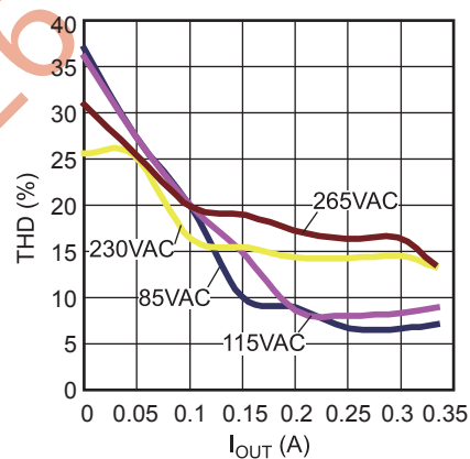
THD vs. I_{OUT}
