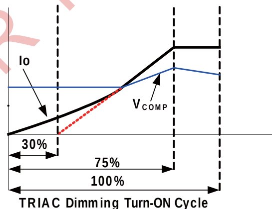
Figure 13: Dimming Curve
