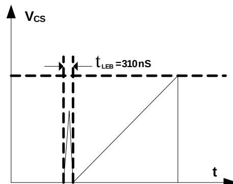
Figure 5: Leading-Edge Blanking
