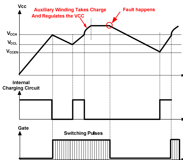
Figure 5: VCC Timing Sequence
