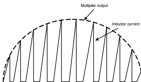
Figure 4: Power-Factor Correction
