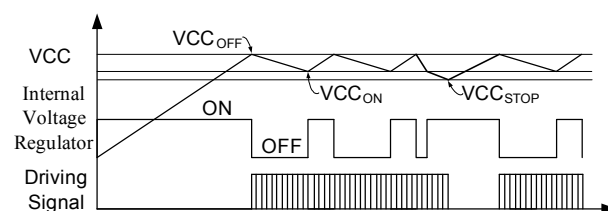
FIGURE 3. VCC Under-Voltage Lock Out (UVLO)
