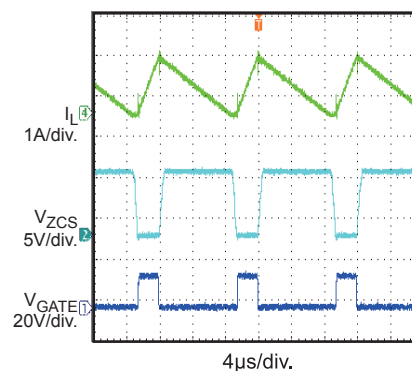
Zero-Current Sensing
