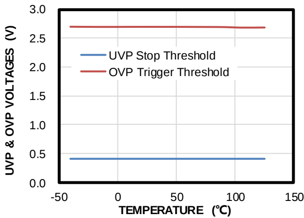
UVP and OVP Voltages vs. T_J
