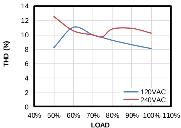
THD
