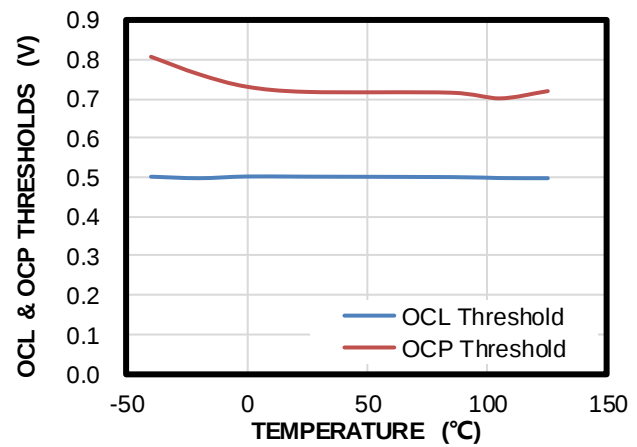
OCL and OCP Thresholds vs. T_J
