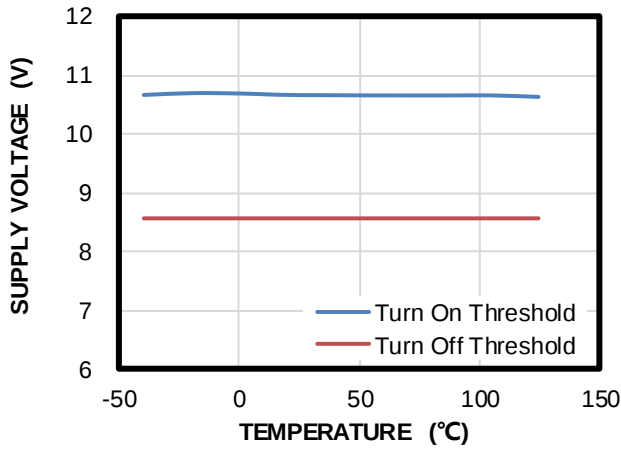
Brown-In and Brownout Voltages vs. T_J
