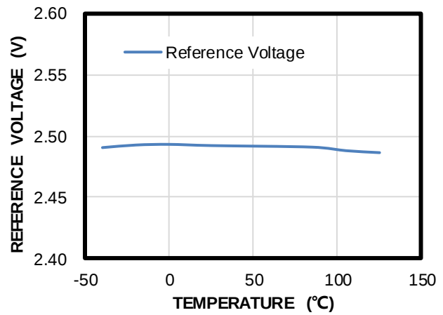
Reference Voltage vs. T_J
