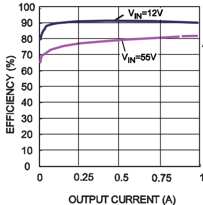
Efficiency @ V_{OUT}=5V
