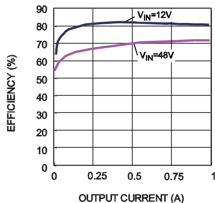
Efficiency @ V_{OUT}=2.5V
