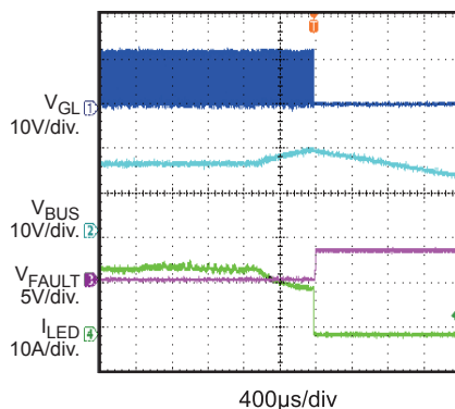
V_{\text{BUS}} OVP Protection
