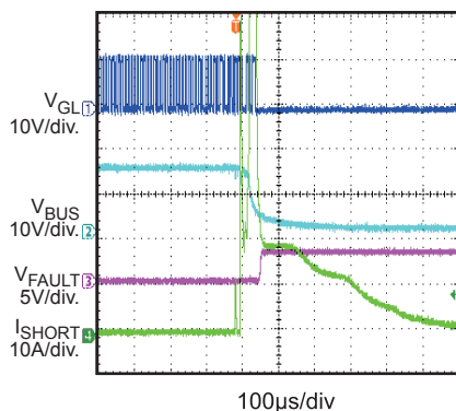
Short V_{\text{BUS}} to GND
